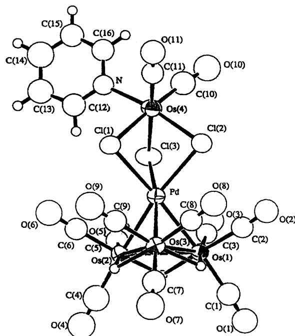
Fig. 5 Molecular structure of [Os_3Pd(CO)_{11}(\mu-H)_3(\mu-Cl)_3(py)] \cdot 0.5C_6H_{14}
