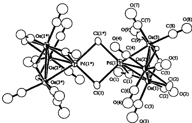
Fig. 4 Molecular structure of [\{Os_3Pd(CO)_9(\mu-H)_2(\mu-Cl)\}_2(\mu-Cl)_2] \cdot H_2O
