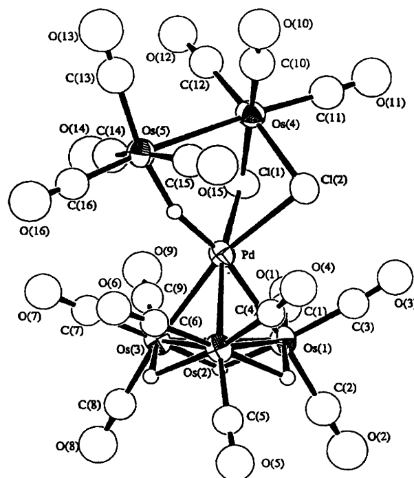
Fig. 3 Molecular structure of [\text{Os}_5\text{Pd}(\text{CO})_{16}(\mu\text{-H})_4(\mu\text{-Cl})_2] 3
