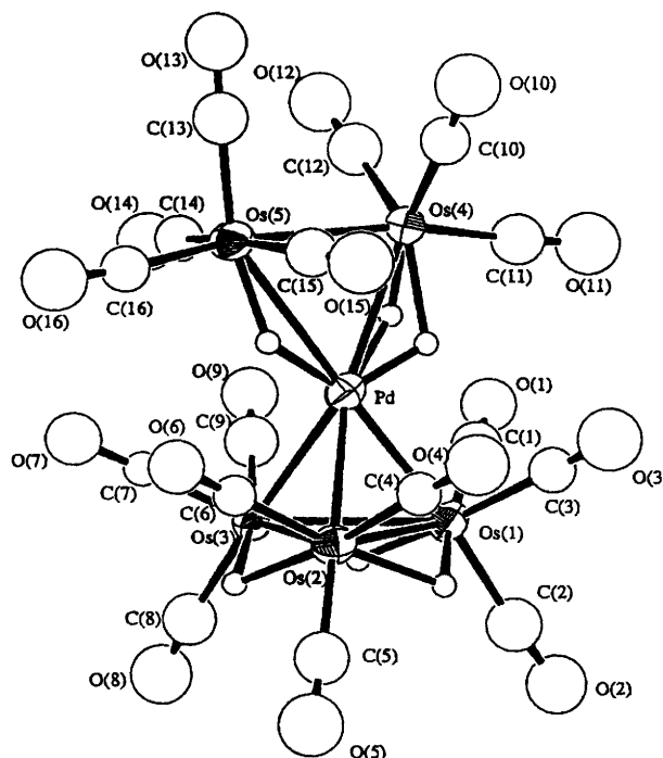
Fig. 1 Molecular structure of [\text{Os}_5\text{Pd}(\text{CO})_{16}(\mu\text{-H})_6] \mathbf{1}
