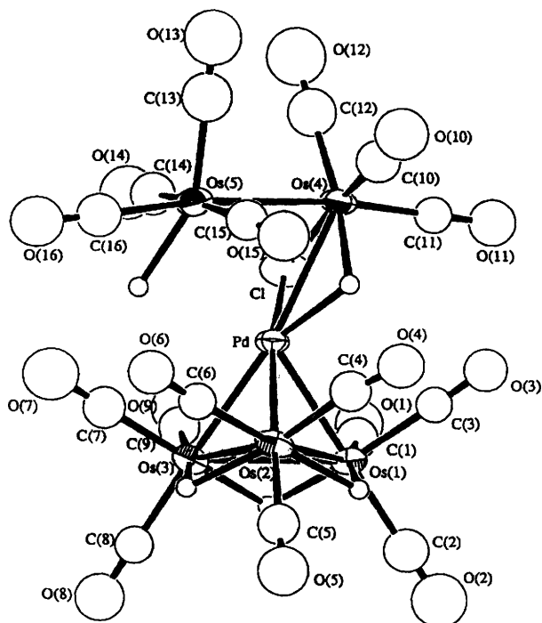
Fig. 2 Molecular structure of [\text{Os}_5\text{Pd}(\text{CO})_{16}(\mu\text{-H})_4\text{H}(\mu\text{-Cl})] 2
